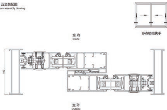
五金装配图 Hardware assembly drawing
