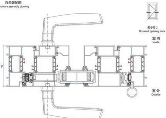
五金装配图 Hardware assembly drawing
