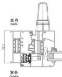
外开窗 Outward opening window
