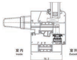
外悬窗 Overhanging window
