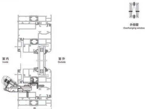
五金装配图 Hardware assembly drawing
