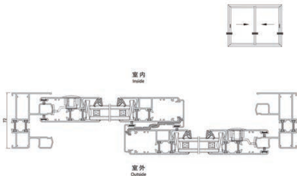
五金装配图 Hardware assembly drawing
